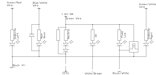
Figure 3. Circuit diagram
