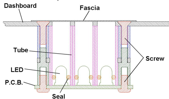
Figure 1 Cross Sectional View
