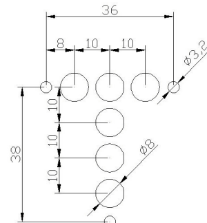
Figure 2. Drill dimensions
